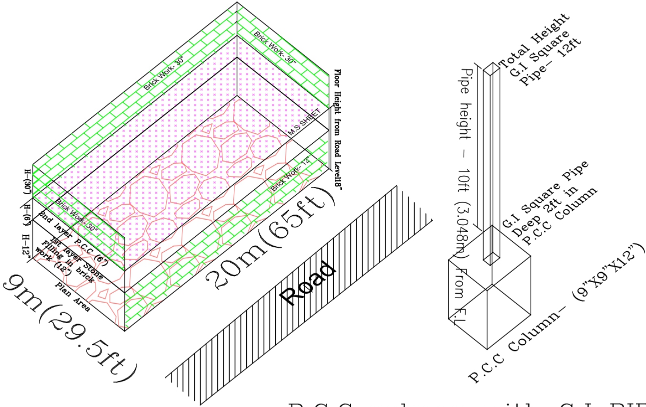
P.C.C column with G.I PIPE
